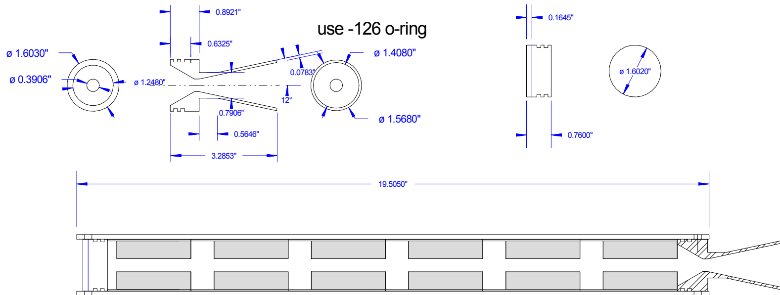
Grain arrangement for SSJ-2 test firing
