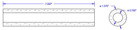
Propellant grain
