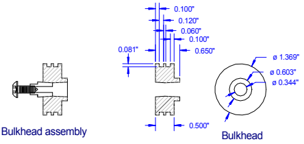
Bulkhead
