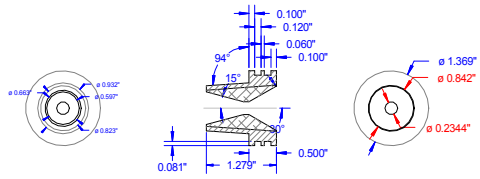
Nozzle assembly
